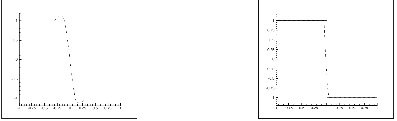
Figure 2.1: Fixed central stencil cubic interpolation (left) and ENO cubic interpolation (right) for the step function. Solid: exact function; Dashed: interpolant piecewise cubic polynomials.
