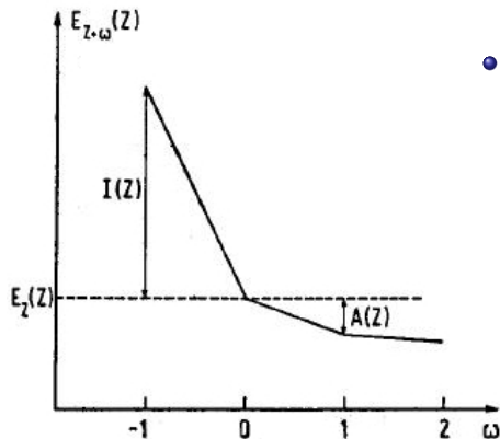
Fig. 2.2. Ground state energy of an atom with nuclear charge Z and (Z+\omega) electrons
